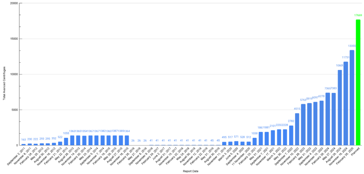
Figure 1. The total number of advanced centrifuges installed at all three enrichment facilities. As can be seen, centrifuge installation accelerated during this reporting period and the previous reporting period, following incremental increases during 2024.
