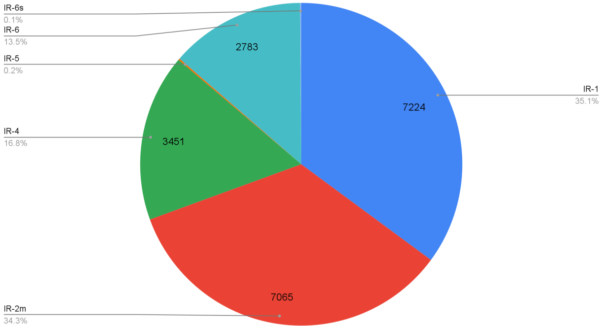
Figure 3. The total number of different types of centrifuges installed by Iran as of February 2025.
