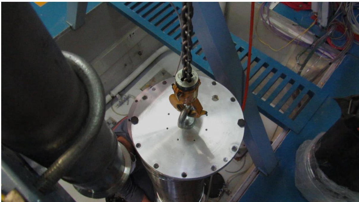
Figure 17. A close-up of the equipment used to lower the centrifuge test machines into the test pit.
