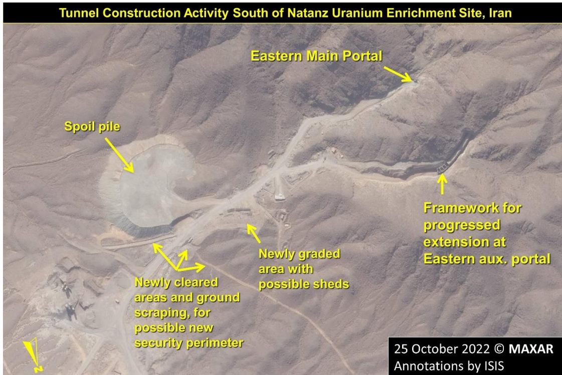
Figure 4. One of the two eastern tunnel portals shows a likely permanent tunnel entrance extension, adding further protection to the entrance. It has progressed in recent months.
