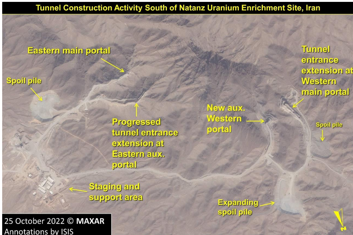
Figure 2. An October 2022 overview image of the tunnel complex shows the new, fourth tunnel entrance (labeled as the “New auxiliary Western portal”)
