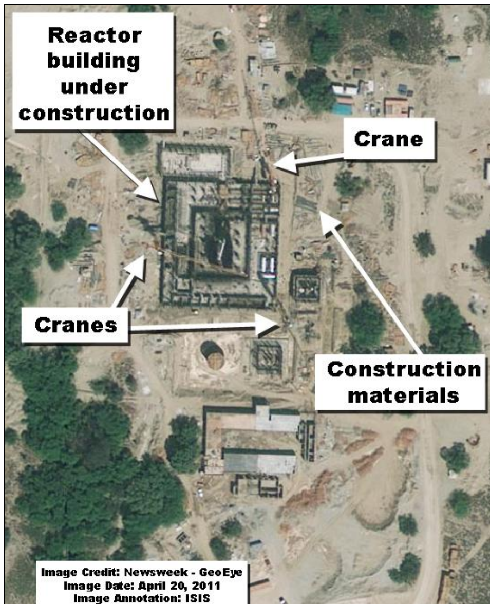
Figure 2. April 20, 2011 image of the construction site for the fourth reactor at the Khushab site. The frame of the building can be seen along with at least three cranes and construction materials surrounding the building.
