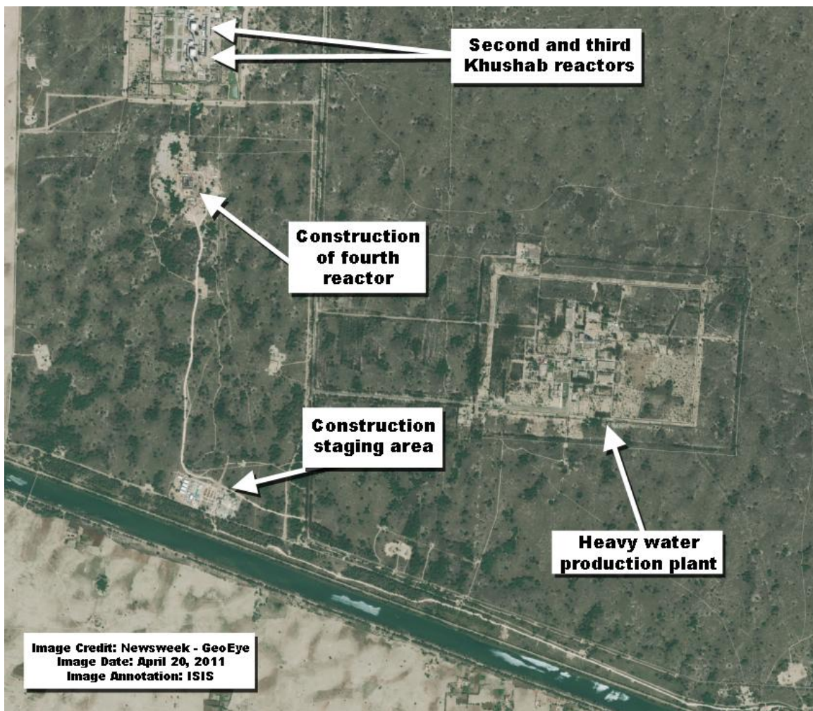
Figure 1. An overview of the southern part of the Khushab nuclear site in Pakistan showing the location of the new reactor construction. The first Khushab reactor cannot be seen in this image. It is located several hundred meters north of the heavy water production plant.
