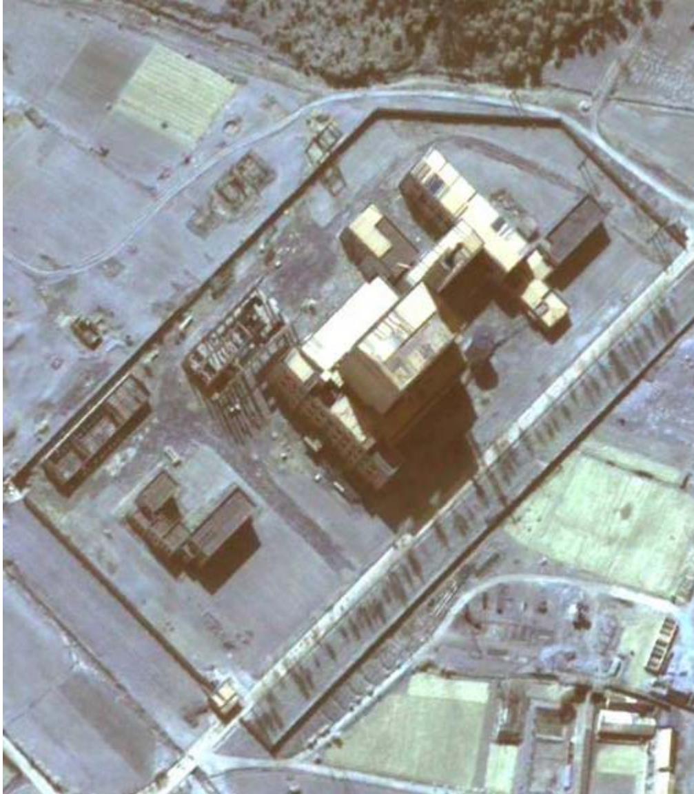
The 50 MWe Reactor Under Construction at Yongbyon
